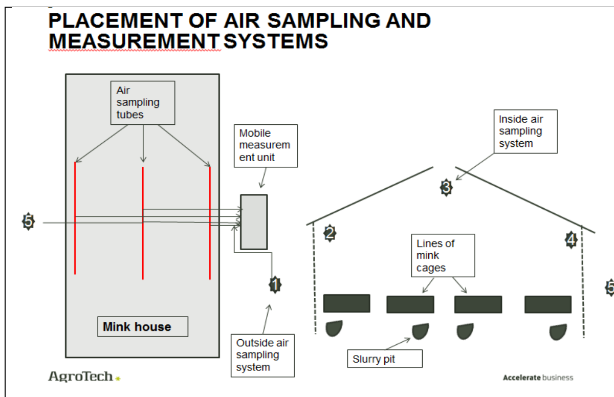
Figure 4. Schematic drawing of the placement of sampling tubes and measurement equipment. Perforated air sampling tubes (20 m long) were situated along the ventilations openings in sides and ridge of the mink house. During sampling, air was drawn by pumps through Teflon tubes from the indoor and outdoor sampling systems to the mobile measurement unit holding the tracer gas measurement system.
